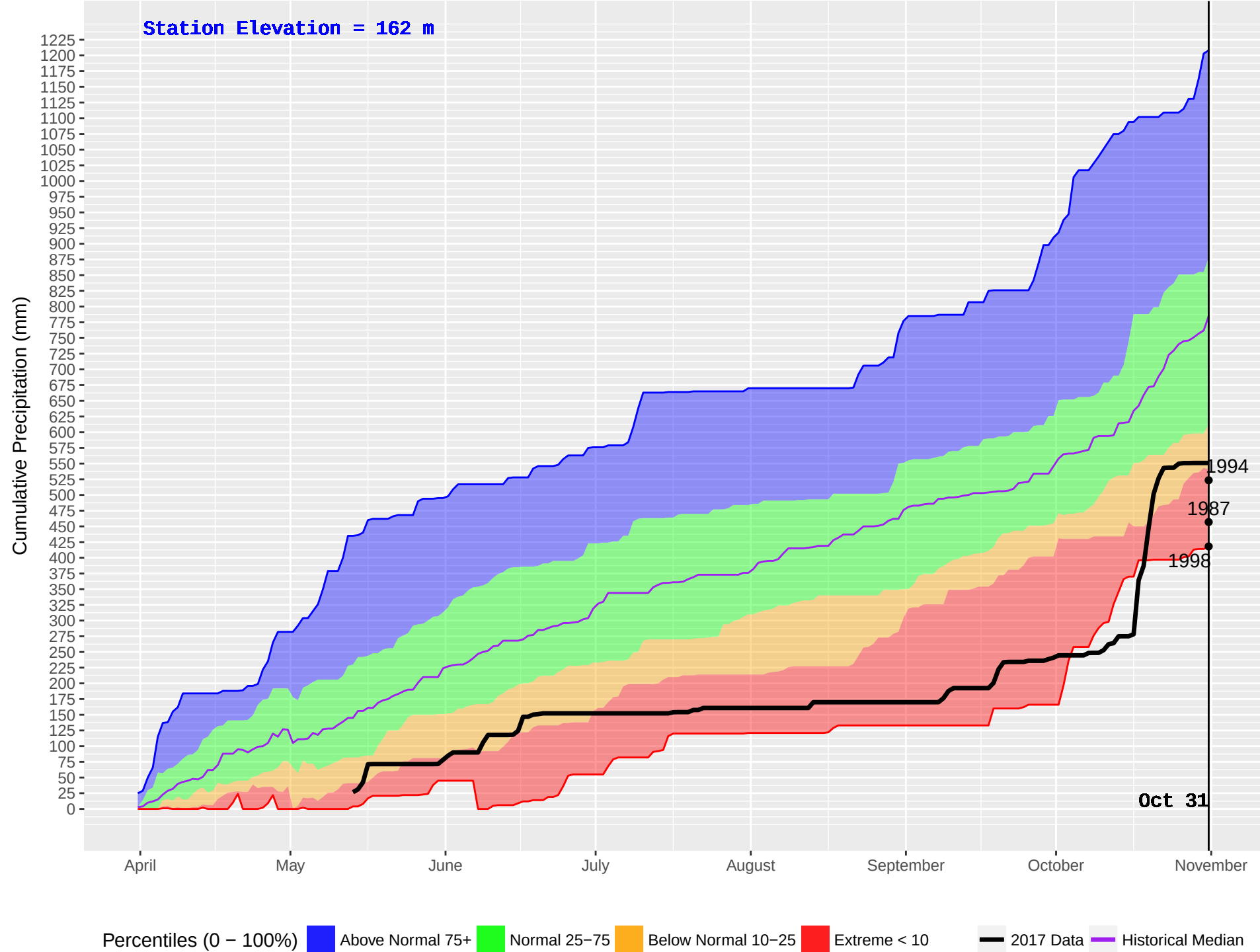
UBC RESEARCH (72) : Historical (1981–2016) and Current (2017) Noon Cumulative Precipitation
